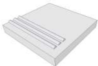
Metal strip inserts fixed into sawn grooves in face of the tread (Available in Stainless Steel or Brass)
